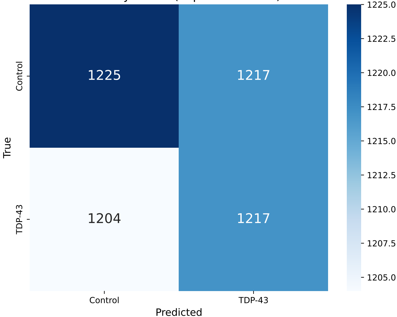
T1 Scrambled Labels - Confusion Matrix Accuracy: 0.502 (Expected: ~0.50)
