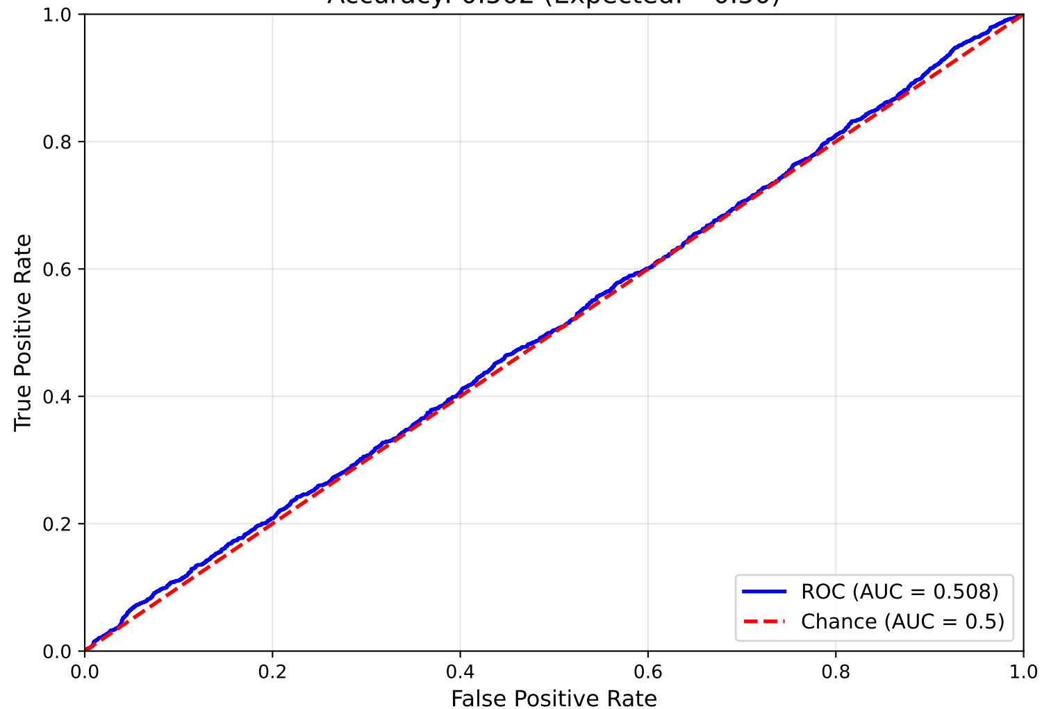
T1 Scrambled Labels - ROC Curve Accuracy: 0.502 (Expected: ~0.50)
