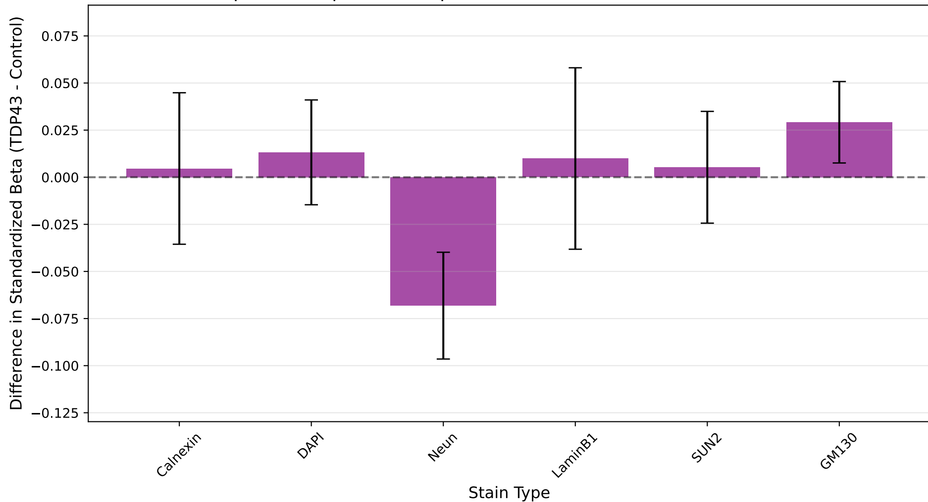
Differential Stain Effects on Gradient (*p<0.05, **p<0.01, ***p<0.001, FDR-corrected Welch's t-test)
