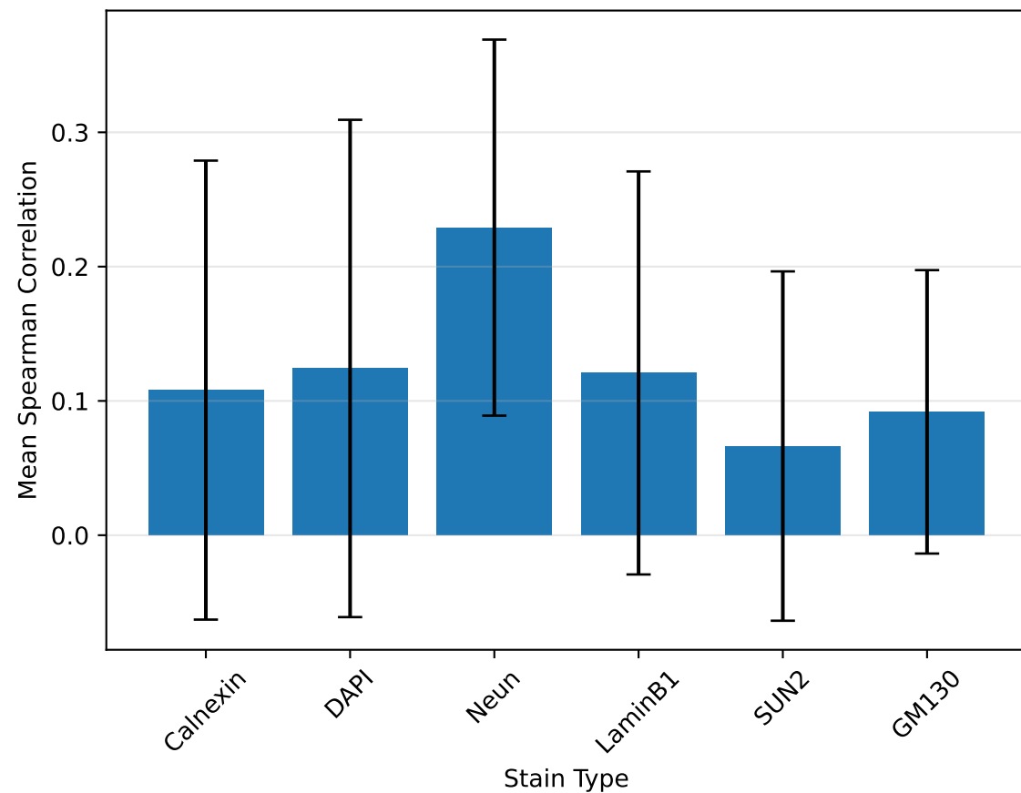
Gradient-Stain Correlations
