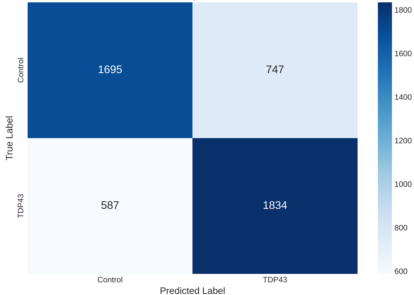
Confusion Matrix Accuracy: 0.726
